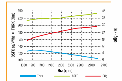
KDI 1903M - PERFORMANS EGRISI
