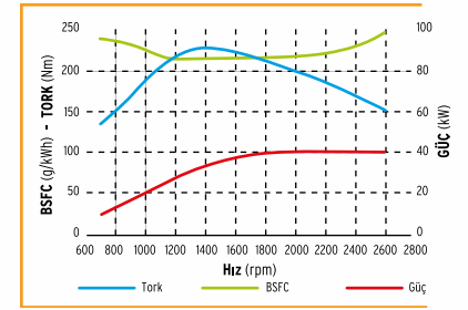
KDI 1903TCR - PERFORMANS EGRISI
